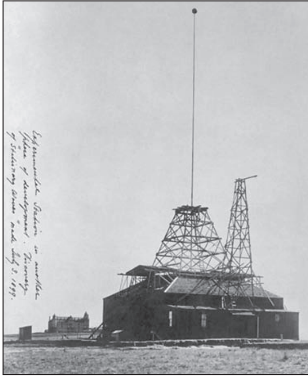
Figure 47. Frontal view of the Colorado Springs laboratory
