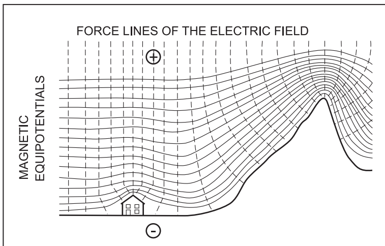
Figure 10. Electric field around an object
