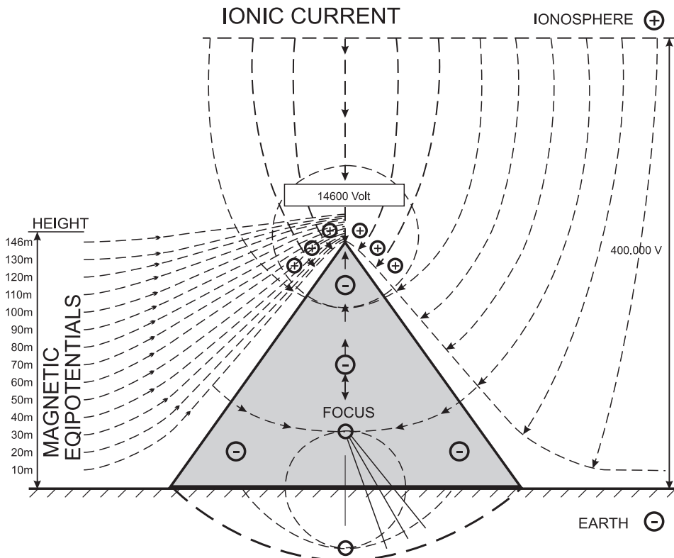
Figure 15. The pyramid's effect on the density of electric and magnetic fields Earth – ionosphere
