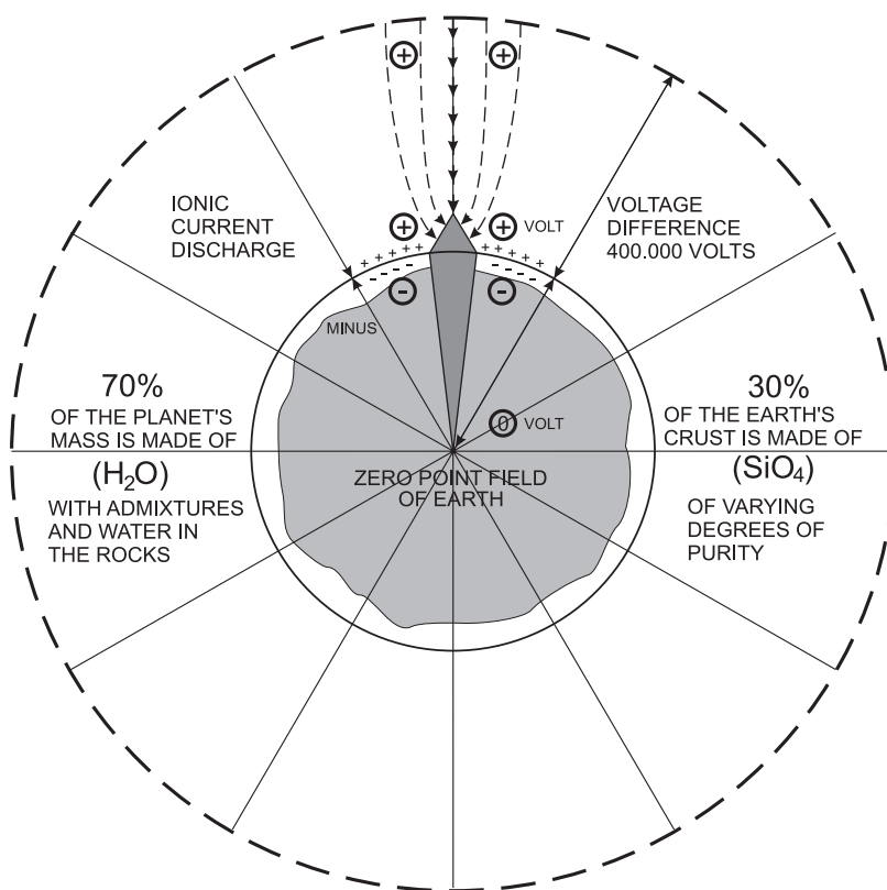
Figure 14. Electric field Earth – ionosphere
