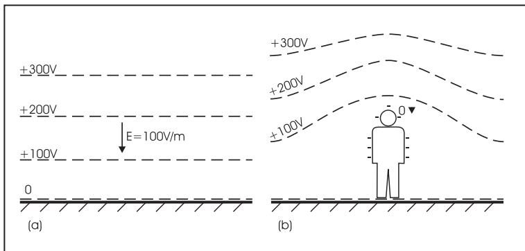
Figure 11. Electric field around a person
