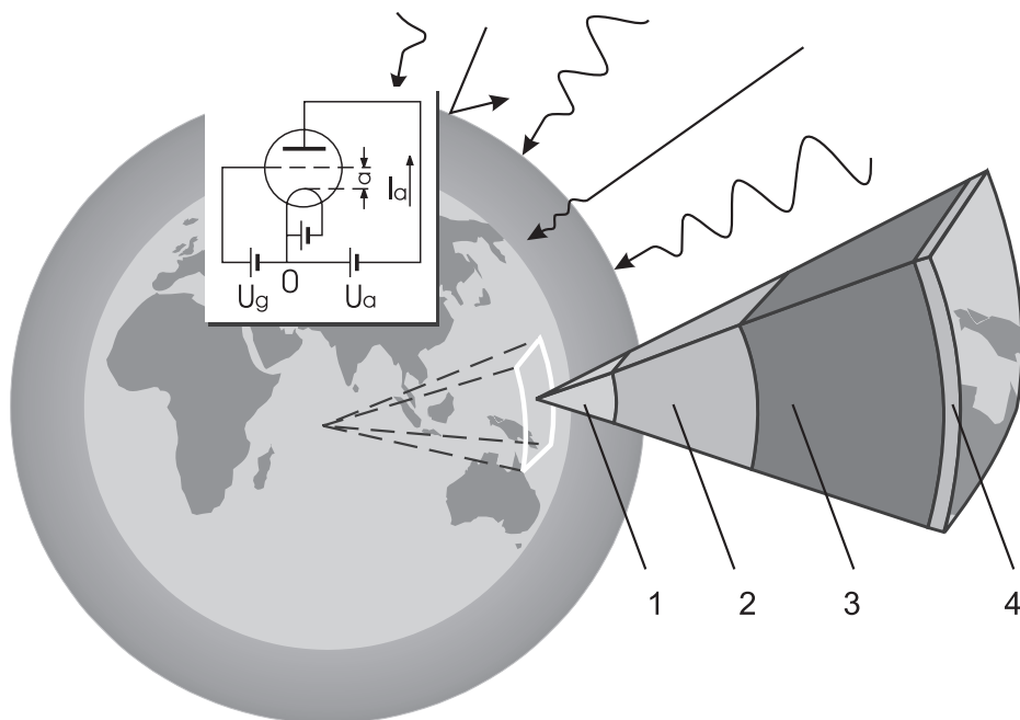
Figure 5. Earth as a spherical capacitor
