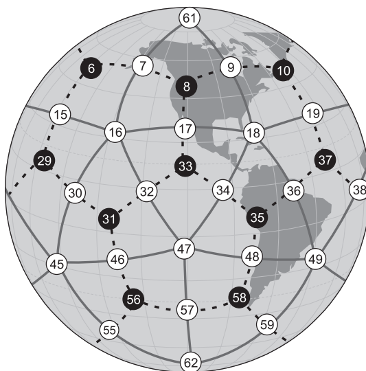
Figure 4a. Icosidodecahedron system of the Earth (IDSZ) on a map of the Earth's hemisphere according to N.F. Goncharov
