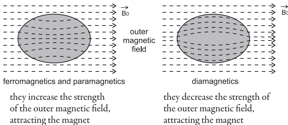
Figure 60. Behavior of paramagnetics and diamagnetics in a magnetic field
