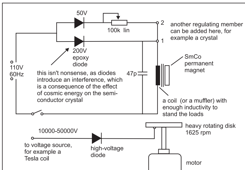
Figure 45. Magnetic resonator
