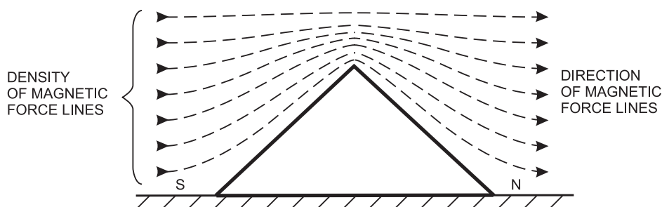
Figure 77. Illustration of the density of magnetic force lines
