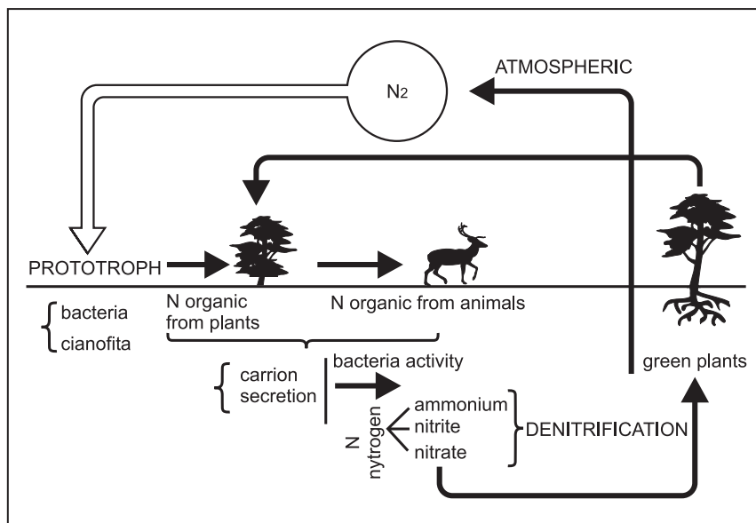
Figure 49. The nitrogen cycle in nature
