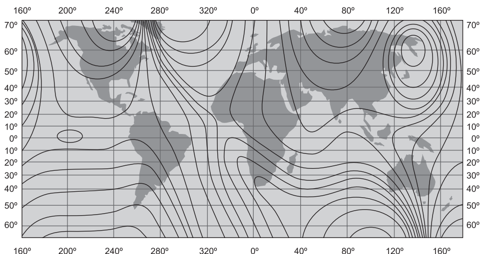
Figure 8. A map of the Earth's magnetic fields and their density
