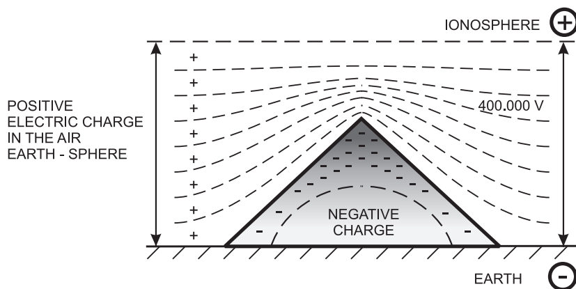
Figure 78. Illustration of the density of electric charges
