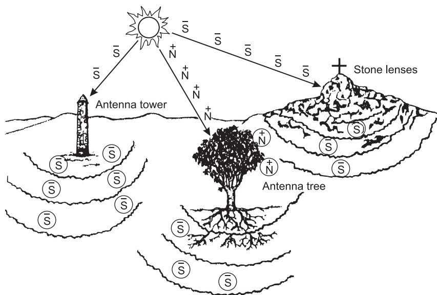
Figure 19. Arrangement of magnetic poles in nature
