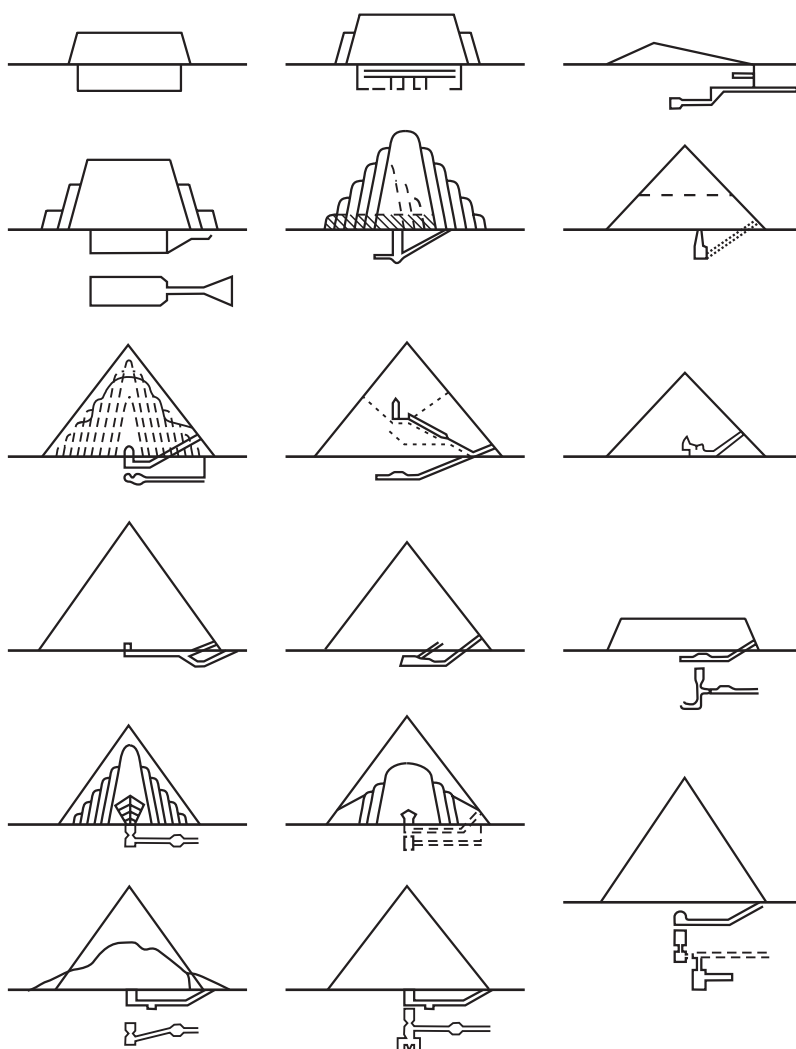
Figure 74. Section of seventeen Egyptian pyramids. The existence of rooms and chambers below the pyramids appears to be a rule.
