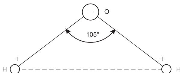
Figure 35. A water molecule
