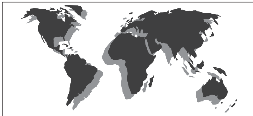
Figure 2. Continental drifts
