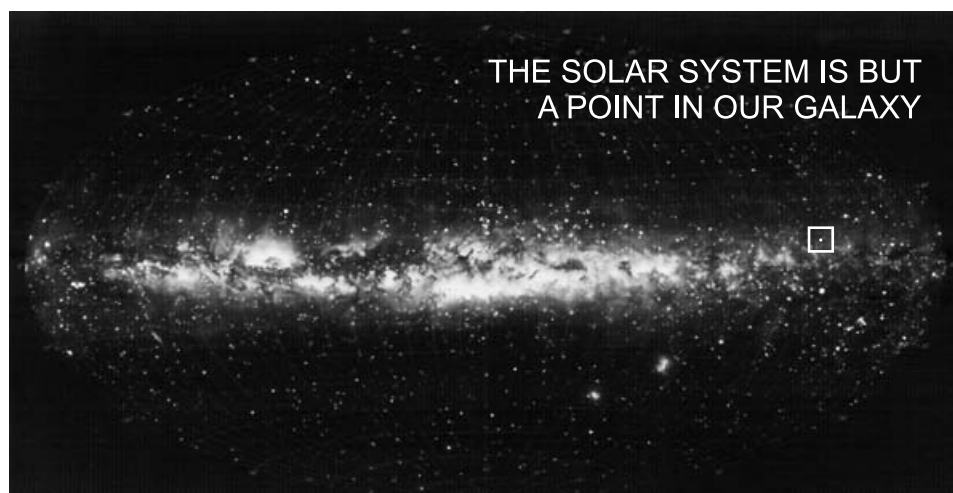
Figure 7. Milky Way
