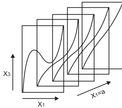
Figure 67. The appearance of function X_3 = X_1^3 - aX_1 for three different cases a < 0 , a = 0 and a > 0 .
