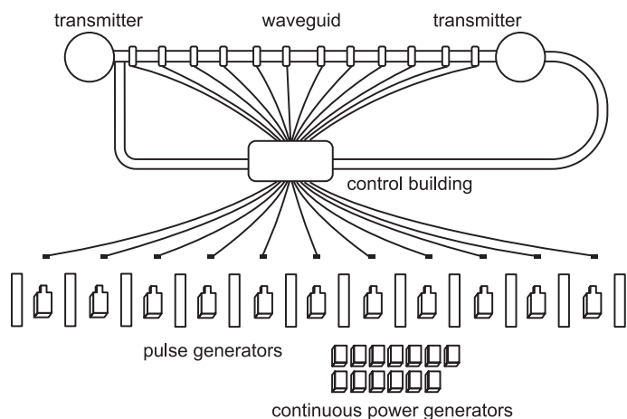
Figure 52. Sketch of the Soviet „Woodpecker“ generator
