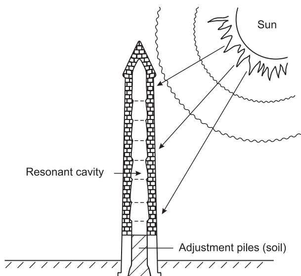
Figure 17. Schematic sketch illustrating the section of an Irish tower
