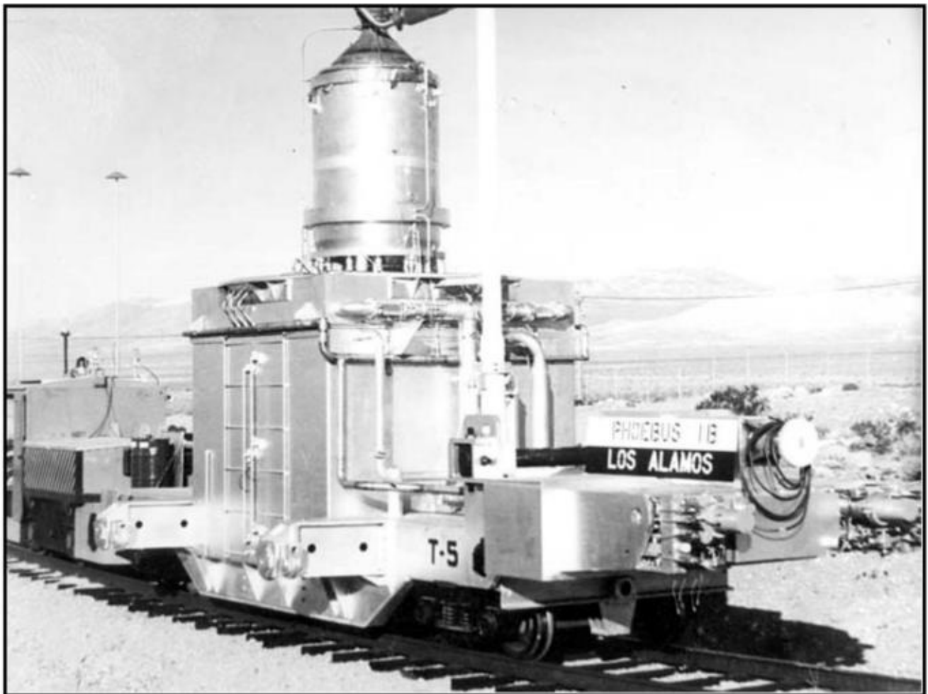
Los Alamos Phoebus I-B on nuclear rocket engine (4,400 Megawatts) at test stand. Courtesy of the U. S.
