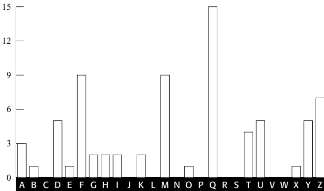
Figure 16 Frequency distribution for letters in the ciphertext encrypted using the L_2 cipher alphabet (number of occurrences).
