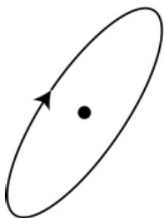
Classical electron orbit
