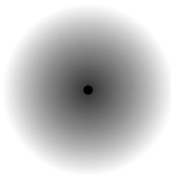
Quantum electron wave function
