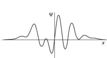
Wave function for one particle with position x
