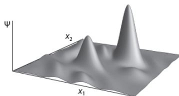
Wave function for two particles with positions x_1, x_2
