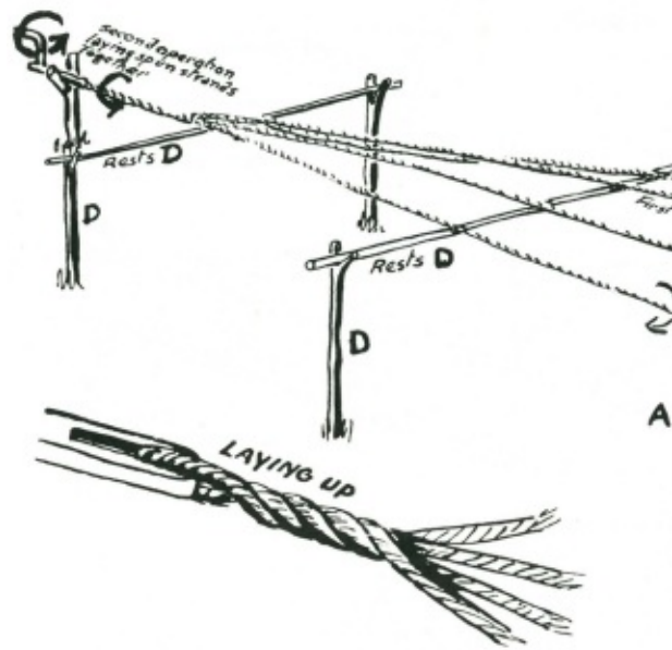
Layout of a rope walk.
