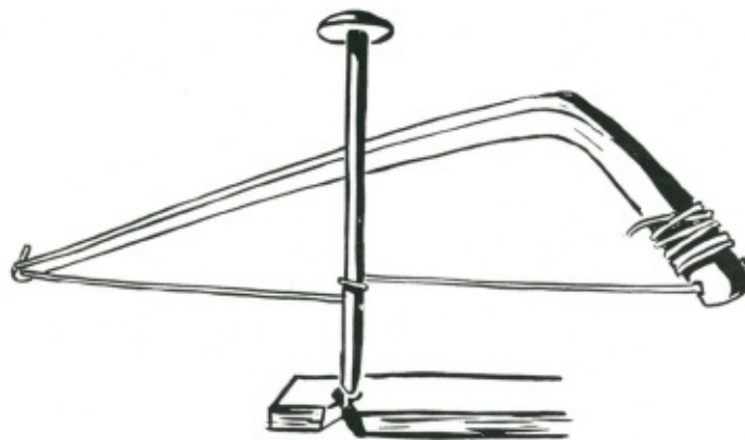
This is how the thong must be round the drill. If the thong is wrong way on the drill it will cross over itself and cut in a few strokes, also the full length of the stroke cannot be obtained.
