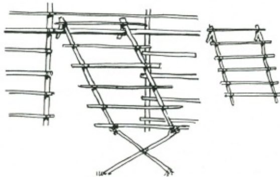
Window frames hook on to thatch batten above window opening.
