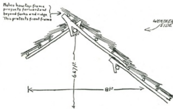
Assembly on framework of sections.
