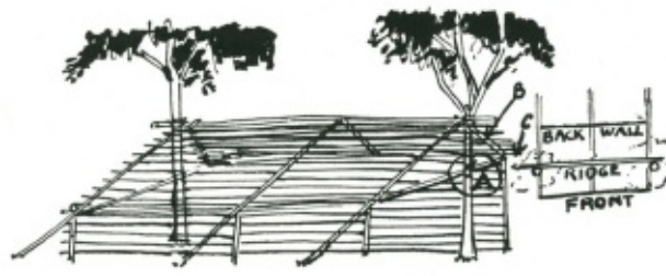
Cutaway section of frame for hut sited between two saplings
