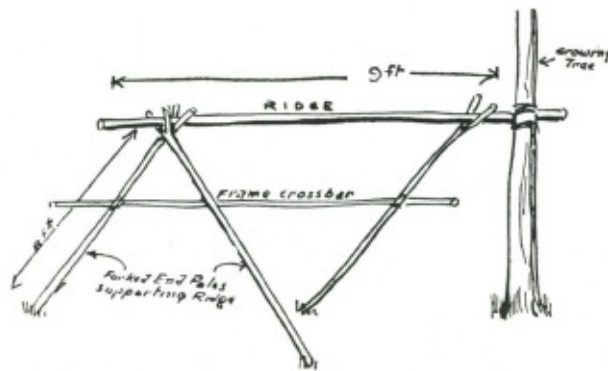
Framework for Sectional Lean-to Shelter
