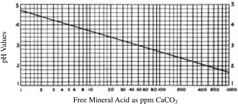
Effect of Mineral Acidity on pH
