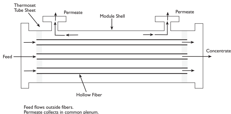
Figure 30 – Hollow Fiber Element
