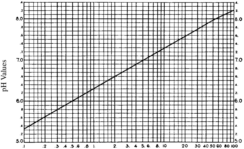
Effect of Bicarbonate Alkalinity and CO 2 on pH
