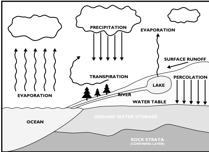
Figure 1 – Hydrologic Cycle
