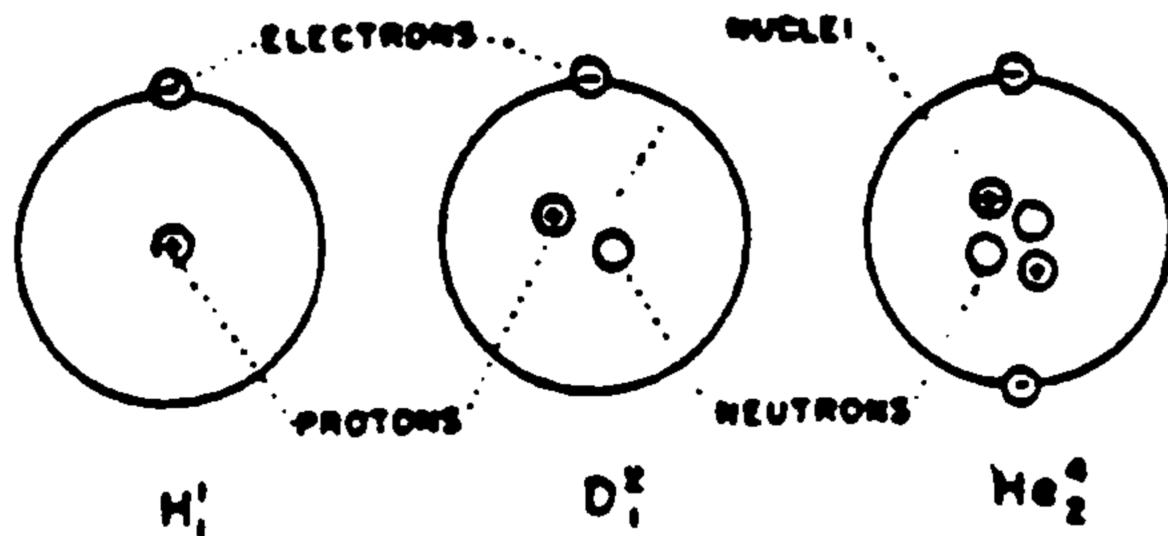
Fig. 2 — Diagram of hydrogen, deuterium and helium atoms.
