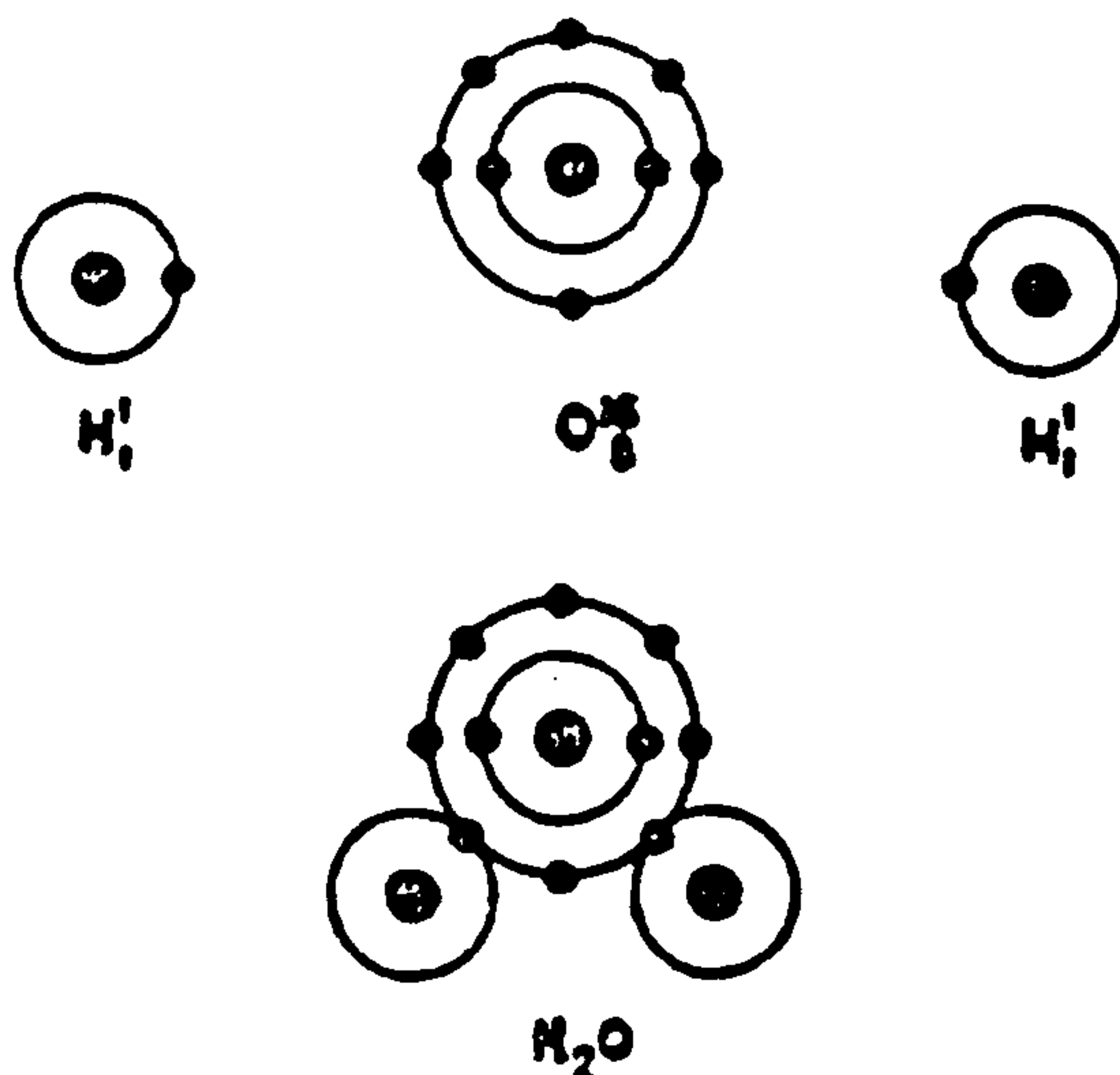
Fig. 3 — Group of oxygen and hydrogen atoms to form H_2O .
