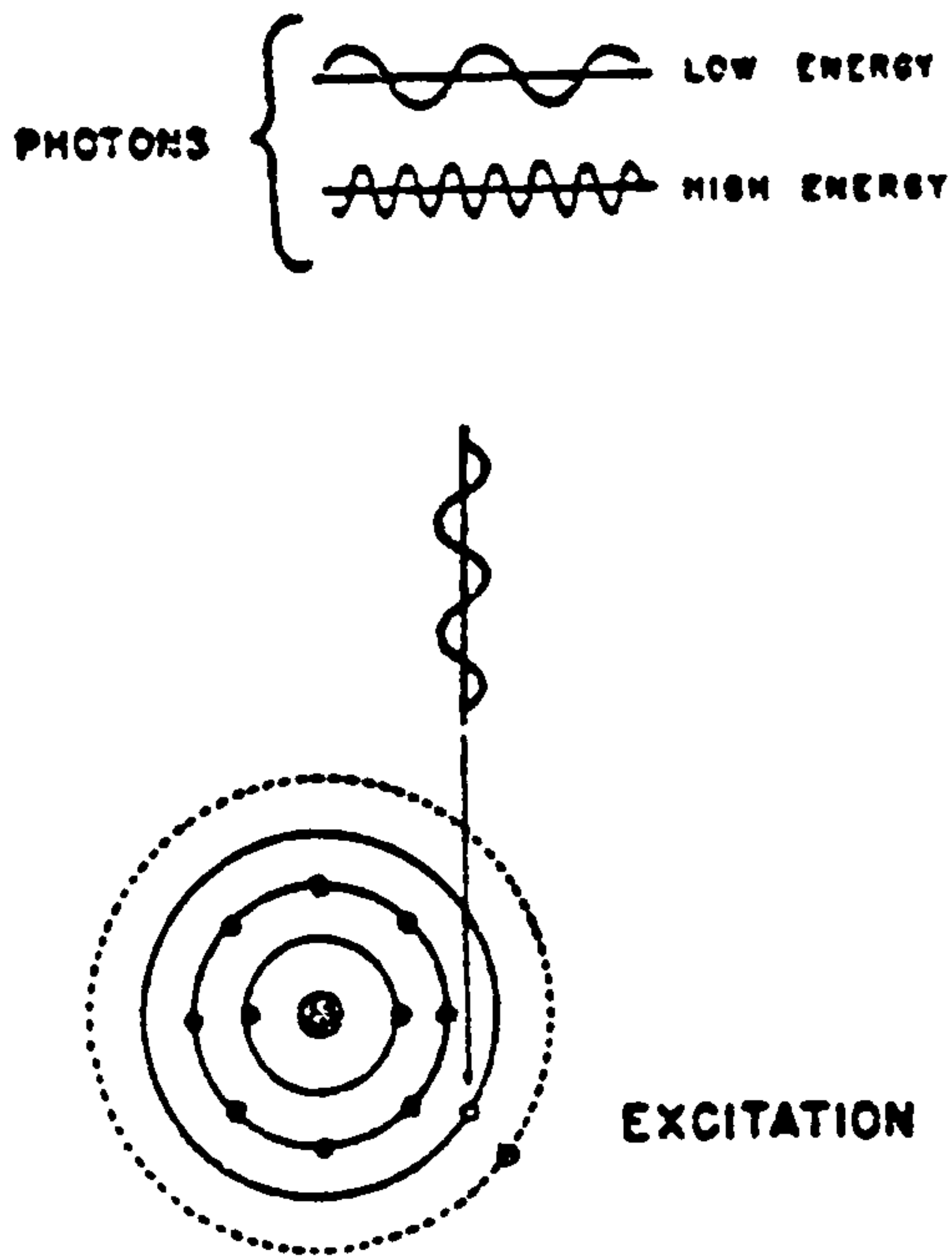
Fig. 4 — Diagram of phenomenon of excitation in the sodium atom.
