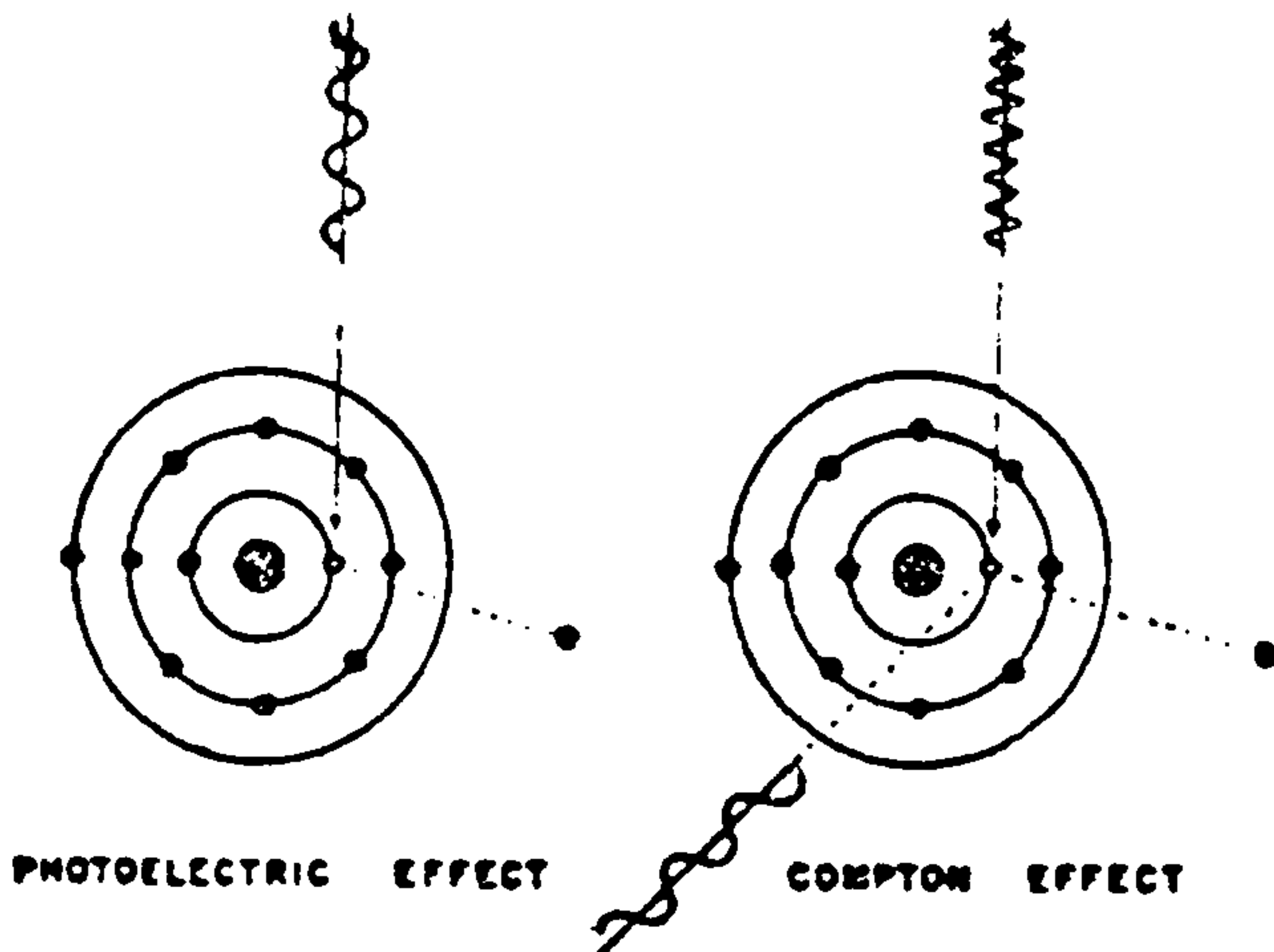
Fig 5 — Diagram of phenomenon of ionization by photoelectric effect and by Compton effect in the sodium atom.
