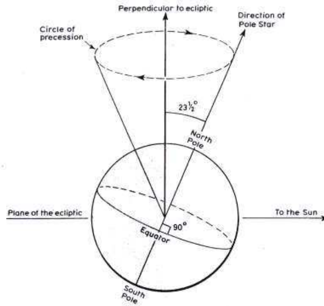
Precession of the Earth's polar axis
