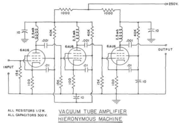
Figure 6-2: Circuit schematic, vacuum tube amplifier for a Hieronymous machine.
