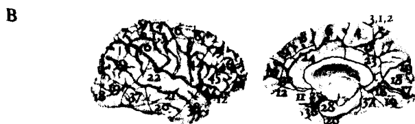
Brodmann's areas
