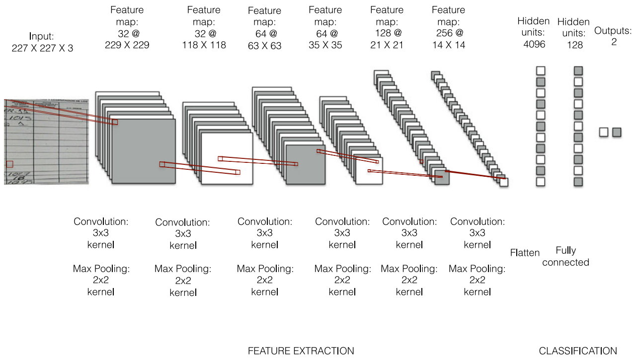
FIGURE 2. Network Architecture
