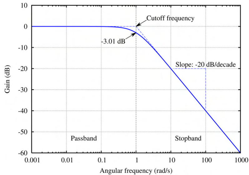
LOW PASS
