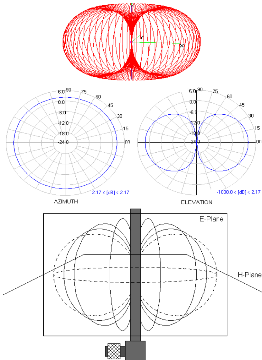
Vertically polarized omnidirectional dipole antenna
