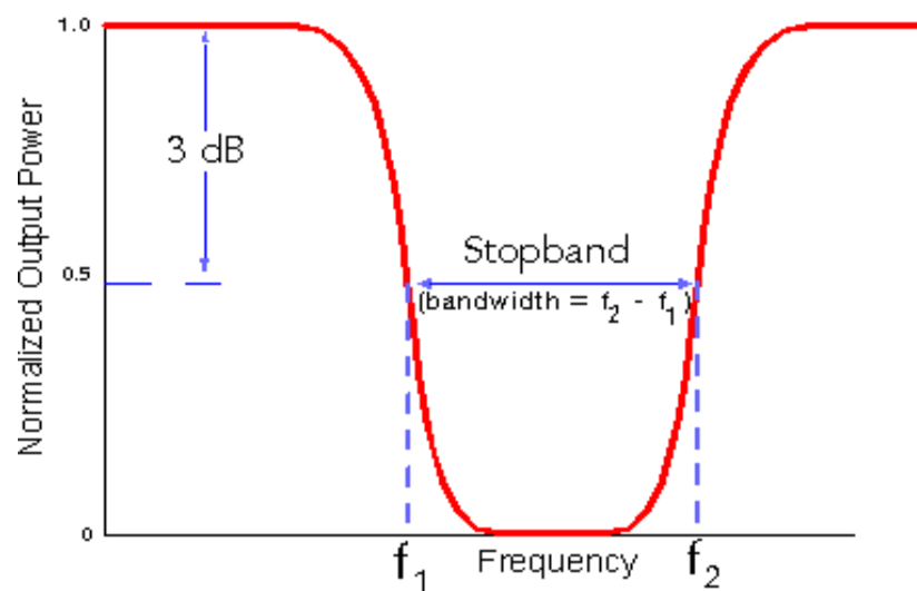
BAND STOP
