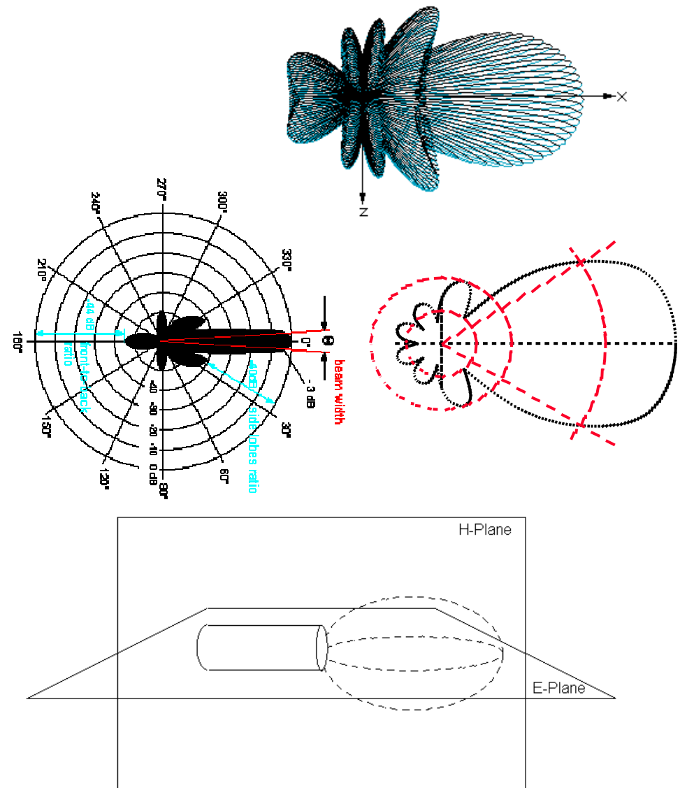
Horizontally polarized directional yagi antenna
