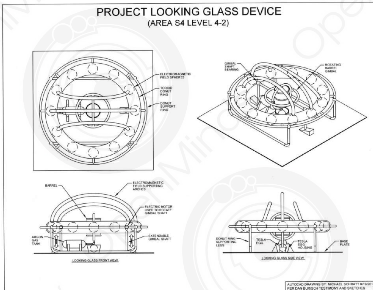
Three-view drawing of the Looking Glass device.*
