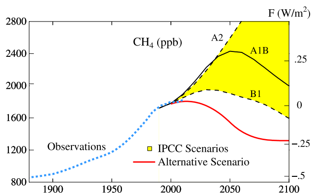
Figure 4. Observed atmospheric CH 4 amount and scenarios for twenty first century. Alternative scenario (Hansen et al 2000, Hansen and Sato 2004) yields maximum global warming ~1.5 °C above 1880–1920. Other scenarios are from IPCC (2001). Forcing on right hand scale is adjusted forcing, F a , relative to values in 2000 (Hansen et al 2007).
