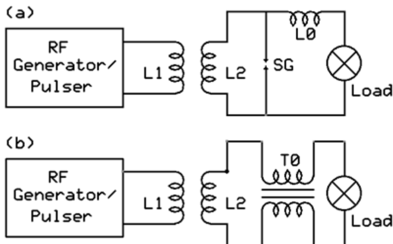
Fig. 6. Reduction of voltage spikes on the load. (a) using a coil, (b) using a toroidal transformer.
