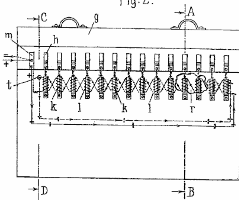
Fig.2 is a face view of the central part of the apparatus.
