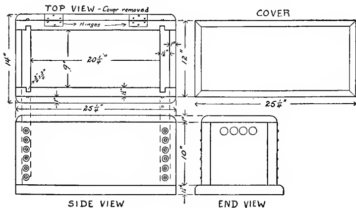
FIG. 31. — TRANSFORMER BOX.
