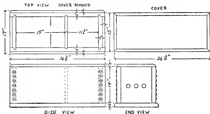
FIG. 32. — HIGH-TENSION BOX.
