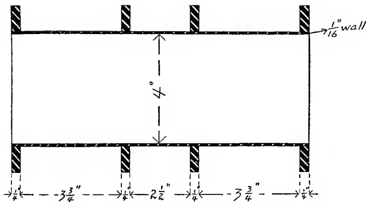
FIG. 39. — SECONDARY BOBBIN OF TRANSFORMER OF 7" COIL.
