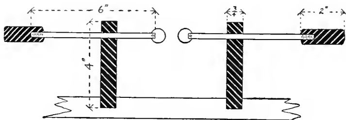
FIG. 47. — PRIMARY SPARK-GAP.
