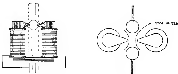
FIG. 17. — MAGNETIC INTERRUPTER.
