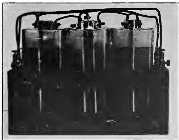
PLATE V. — The Electrolytic Rectifier.
