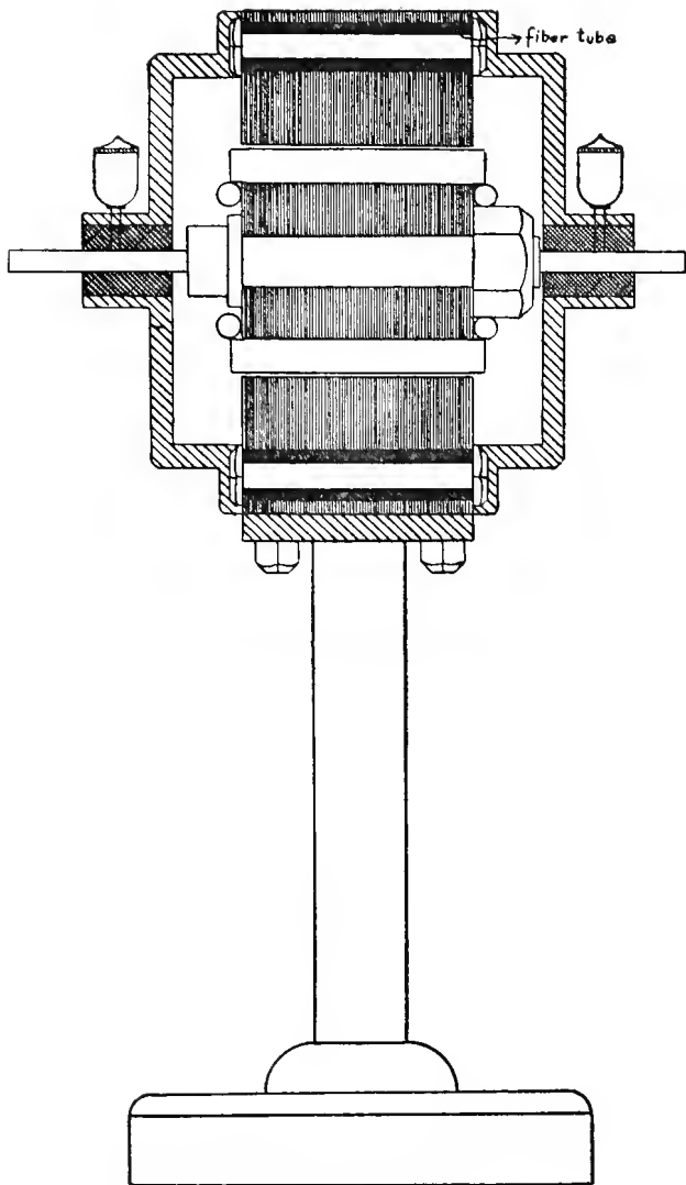
FIG. 24. — SECTION OF COMPLETED MOTOR.
