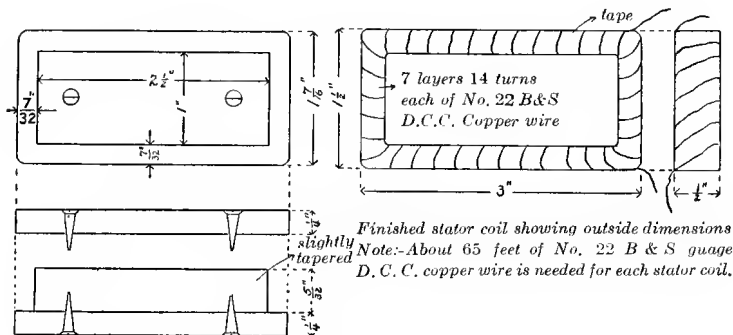
Frame on which stator coils are wound.
