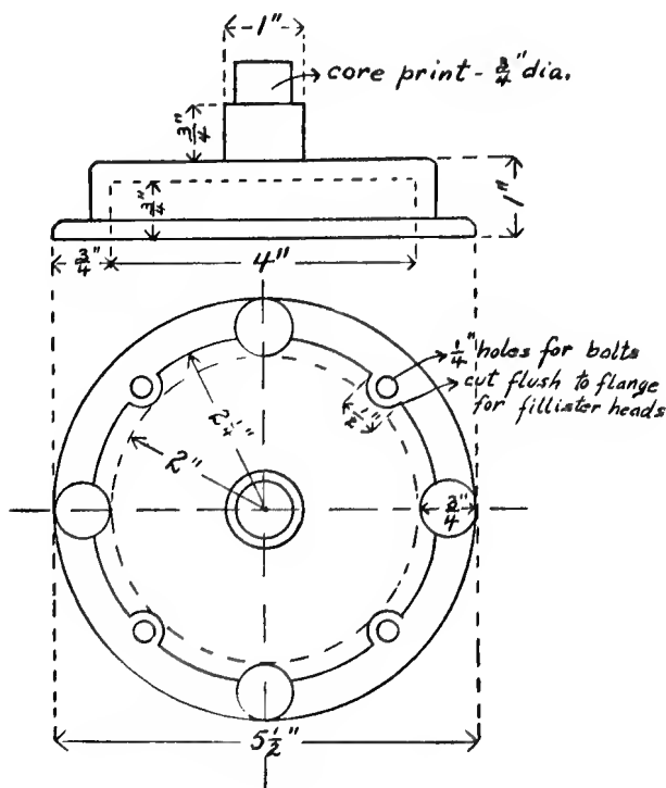
FIG. 23. — PATTERN OF YOKE.
