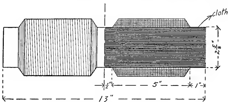
FIG 38. — PRIMARY AND CORE OF TRANSFORMER OF 7" COIL.
