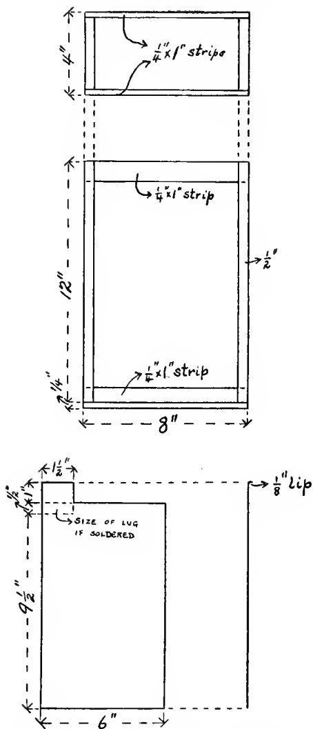
FIG. 40. — PLATE AND FRAME OF CONDENSER.
