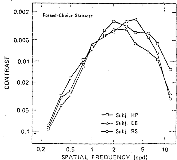
Fig. 6. Contrast sensitivity vs spatial frequency for three young, emmetropic Ss, obtained by the FCS technique.
