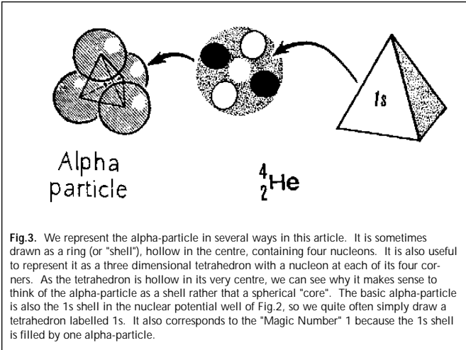
Fig. 3. We represent the alpha-particle in several ways in this article. It is sometimes drawn as a ring (or "shell"), hollow in the centre, containing four nucleons. It is also useful to represent it as a three dimensional tetrahedron with a nucleon at each of its four corners. As the tetrahedron is hollow in its very centre, we can see why it makes sense to think of the alpha-particle as a shell rather than a spherical "core". The basic alpha-particle is also the 1s shell in the nuclear potential well of Fig. 2, so we quite often simply draw a tetrahedron labelled 1s. It also corresponds to the "Magic Number" 1 because the 1s shell is filled by one alpha-particle.
