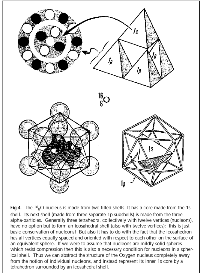
Fig. 4. The ^{16}_8\text{O} nucleus is made from two filled shells. It has a core made from the 1s shell. Its next shell (made from three separate 1p subshells) is made from the three alpha-particles. Generally three tetrahedra, collectively with twelve vertices (nucleons), have no option but to form an icosahedral shell (also with twelve vertices): this is just basic conservation of nucleons! But also it has to do with the fact that the icosahedron has all vertices equally spaced and oriented with respect to each other on the surface of an equivalent sphere. If we were to assume that nucleons are mildly solid spheres which resist compression then this is also a necessary condition for nucleons in a spherical shell. Thus we can abstract the structure of the Oxygen nucleus completely away from the notion of individual nucleons, and instead represent its inner 1s core by a tetrahedron surrounded by an icosahedral shell.
