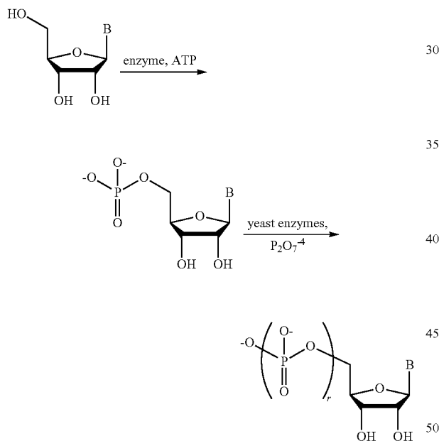
Scheme 10
