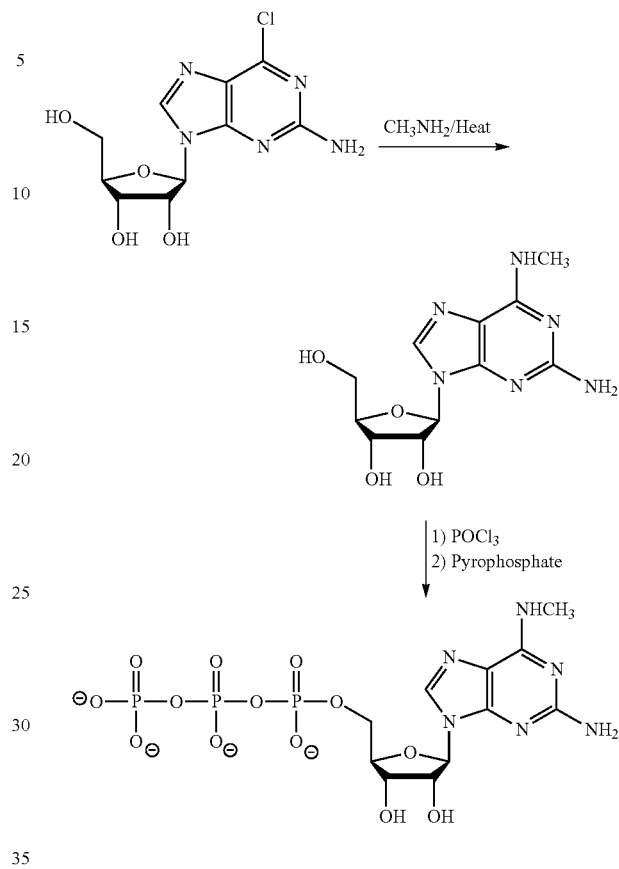
Scheme 7
