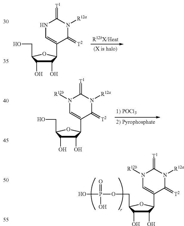
Scheme 11
