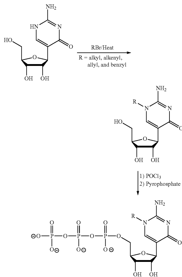
Scheme 6
