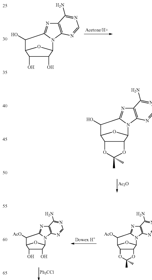
Scheme 2
