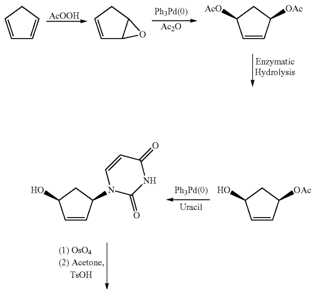
Scheme 8
