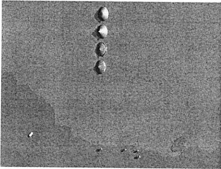
Fig. 4 Rendering using a sun position derived from the photograph.
